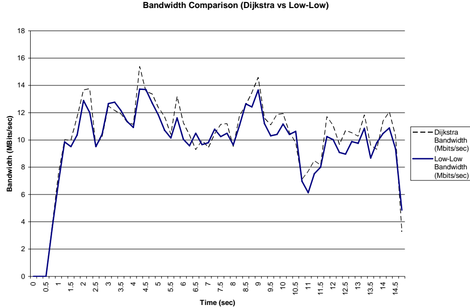
Figure 9. Bandwidth (Dijkstra vs Low-Low)
